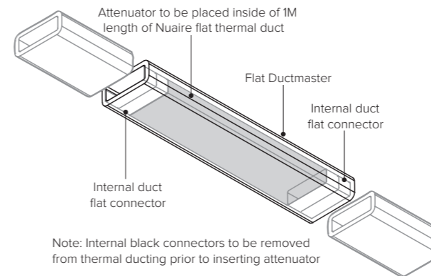
FIGURE 8: TYPICAL RECTANGULAR THERMAL DUCT WITH AN ATTENUATOR
